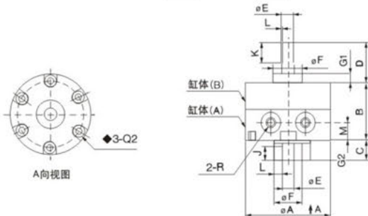
CRB2BW10-□S (通口在缸体侧面)
